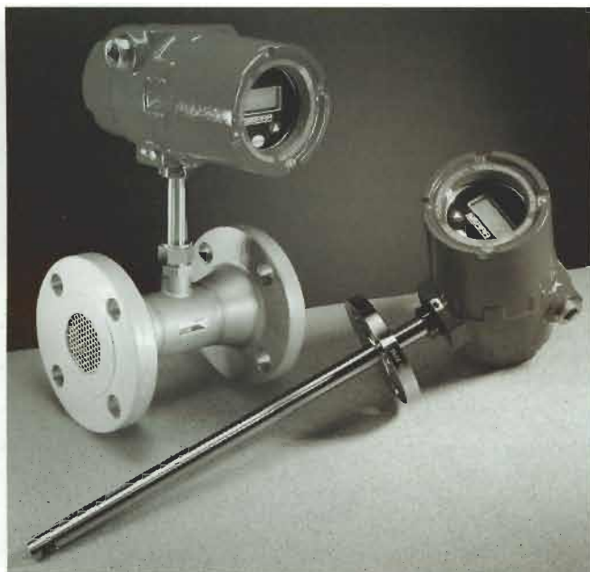
FIGURE 2. Industrial thermal mass flowmeters are available in both insertion and in-line configurations.
