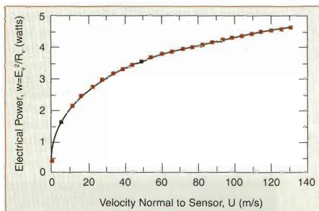
FIGURE 3. Typical flow calibration curve for an industrial thermal mass flowmeter. The electronics drive is that shown in Figure 1. The constant temperature differential ( T_v - T_f ) is 50.0^\circ\text{C} . The cold resistances R_{v0} and R_{f0} of the velocity and temperature sensors at 20^\circ\text{C} are approximately 20 and 200\Omega , respectively.
