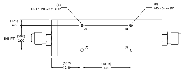
C180H, H1, H2 Bottom View
