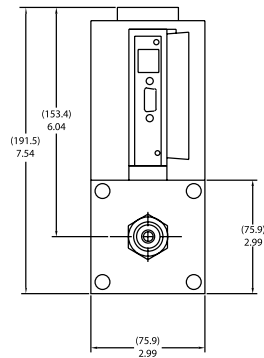
C100H, H1, H2 Side View
