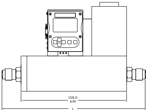
C100H, H1, H2 Front View
