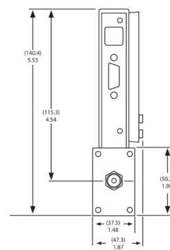
C100M Inlet View
