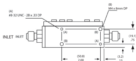
M100L & C100L Bottom View
