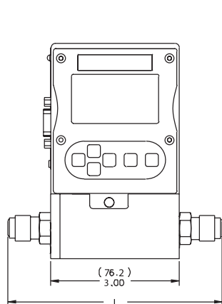
M100L & C100L Front View
