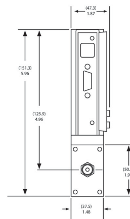
C100M Inlet View
