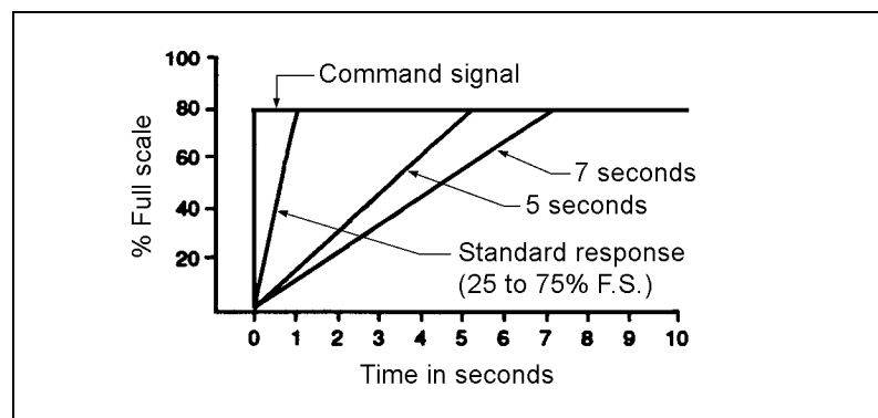
Figure 3-1. Soft Start Response Times
