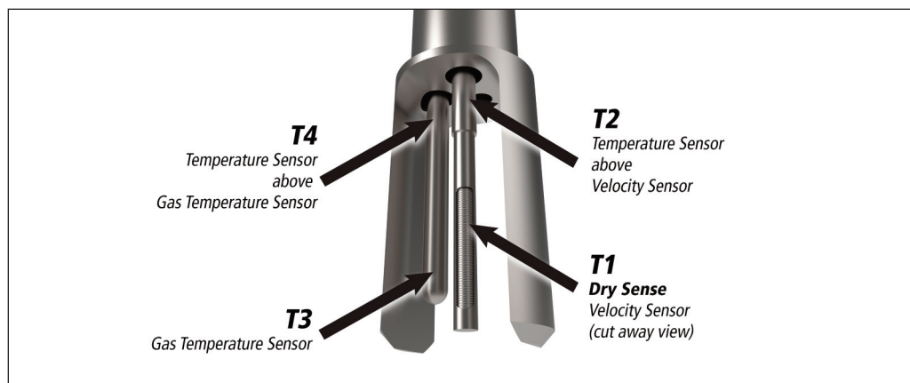
Figure 3. DrySense Velocity Sensor
