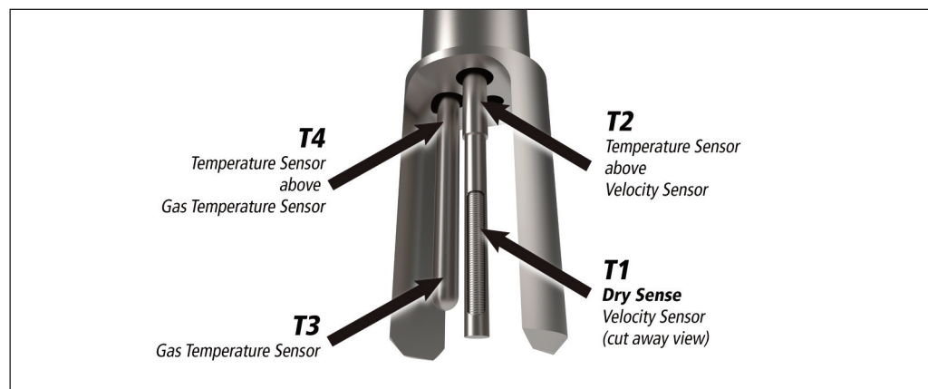
Figure 2. New QuadraTherm "Four-Sensor" Thermal Dispersion Flow Sensor
