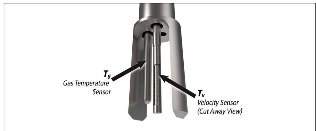
Figure 1. Traditional “Two-Sensor” Thermal Dispersion Flow Sensor
