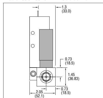
Model 830M/840M — Outlet View
