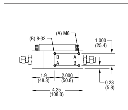
Model 830M/840M — Bottom View
