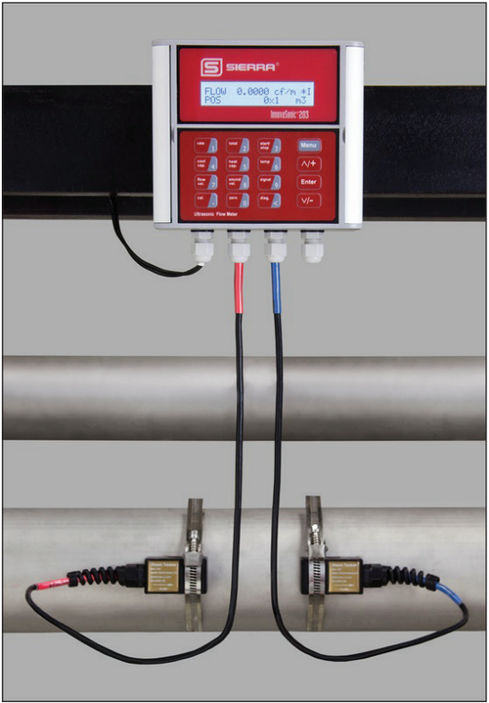
Installing the Transducers (example)
