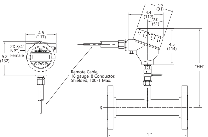
745i Inline Remote Meter - 300 lb Flange
