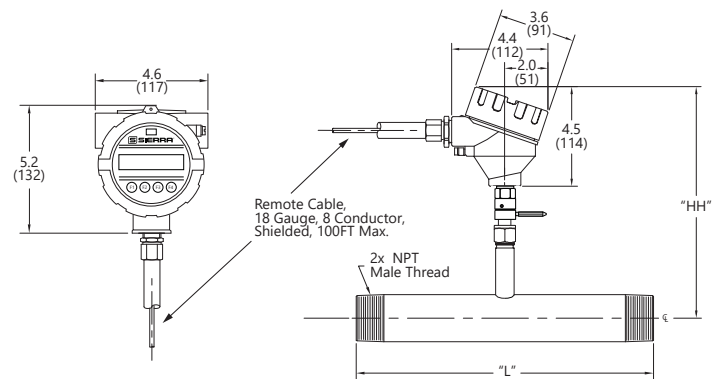
745i Inline Remote Meter - NPT
