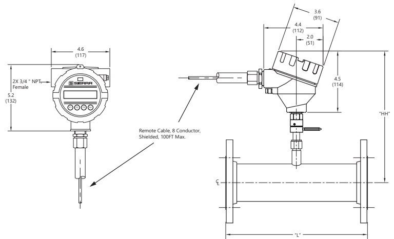
745i Inline Remote Meter - 150 lb Flange
