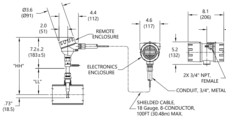
645i Insertion Remote Meter
