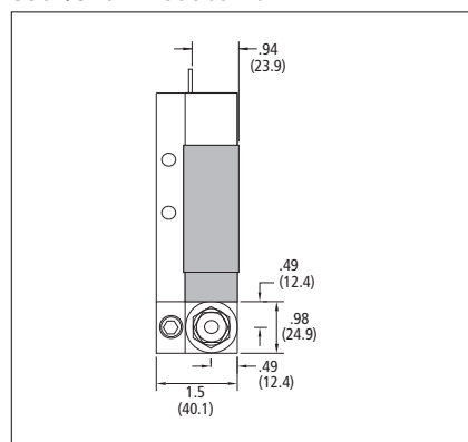
830L/840L — Outlet View
