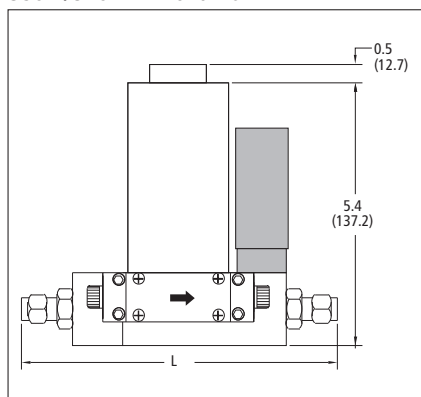
830M/840M — Front View
