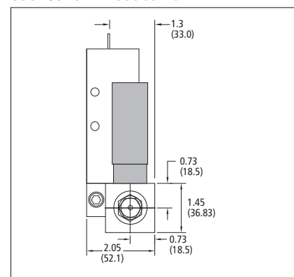
830M/840M — Outlet View
