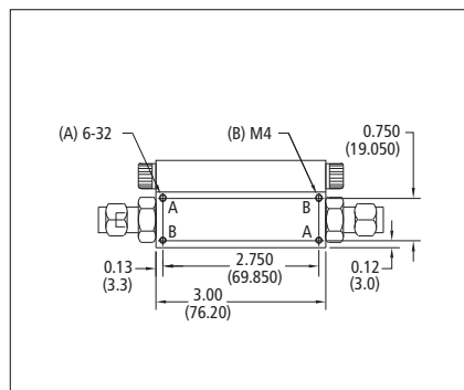
830L/840L — Bottom View
