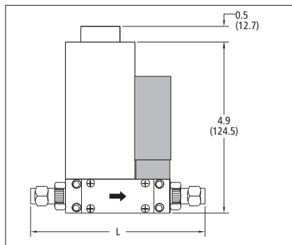
830L/840L— Front View
