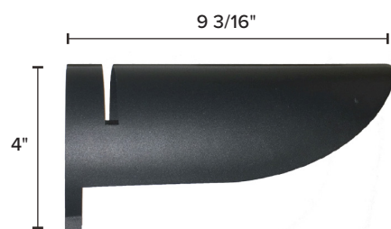
Figure A: Sun Shade Dimensions
