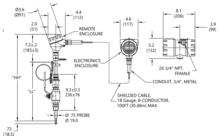
Insertion Remote Meter with Hot-Tap
