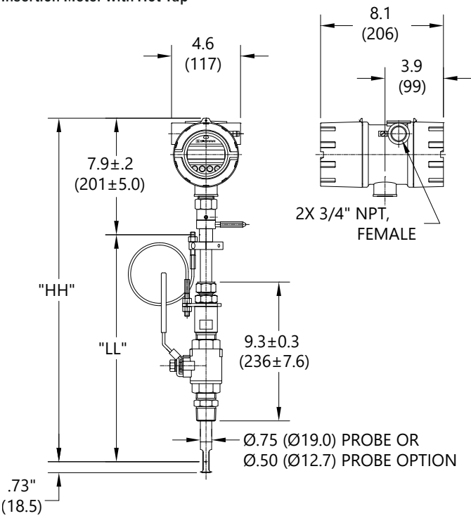
Insertion Meter with Hot-Tap
