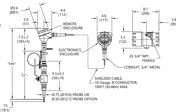
Insertion Remote Meter with Hot-Tap
