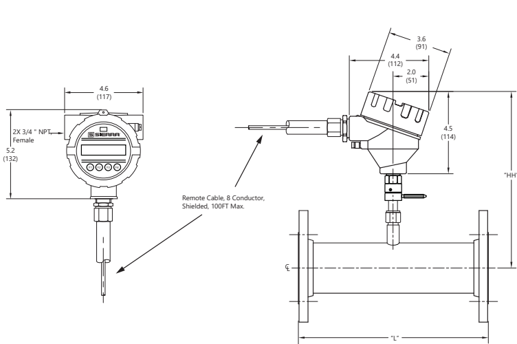
Inline Remote Meter - 150 lb Flange
