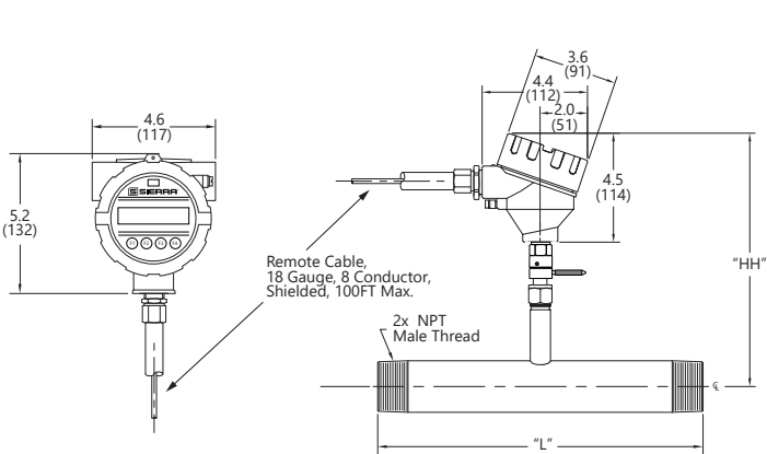
Inline Remote Meter - NPT
