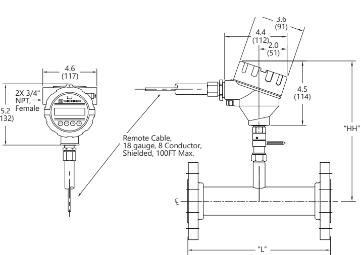
Inline Remote Meter - 300 lb Flange
