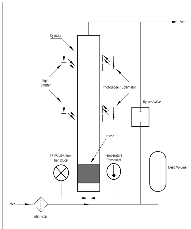
Figure 1: DryCal 1020 & 1500 Operating Principle
