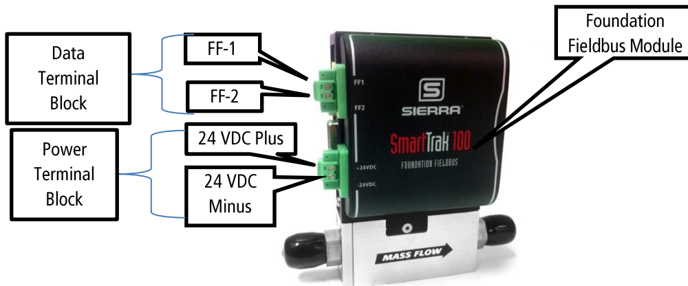
Figure 1: Connection Points
