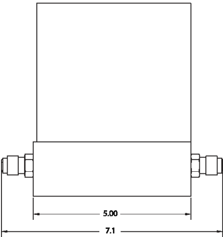
50 Series - Bottom View
