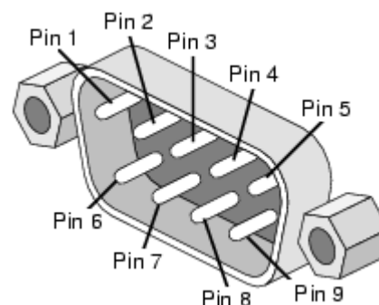
Figure: DB9 Pin-out (There are two DB9 connectors, one on each side of the enclosure. Assure block off plate covers unused DB9).
