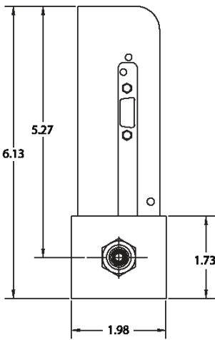
50 Series - Side View
