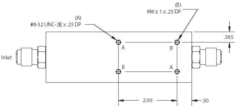
50 Series - Bottom View
